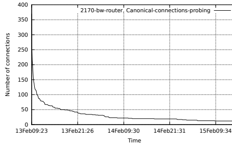
Fig. 6. Persistent connections decay rate for a random router
