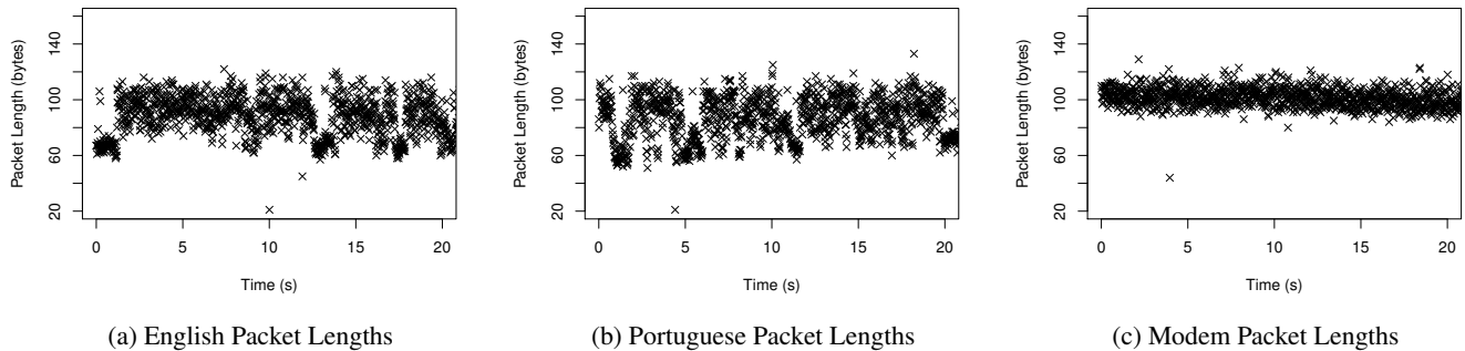
Figure 9: Skype packet lengths of English and Portuguese speech samples from the OPI corpus compared to modem audio sent over Skype.
